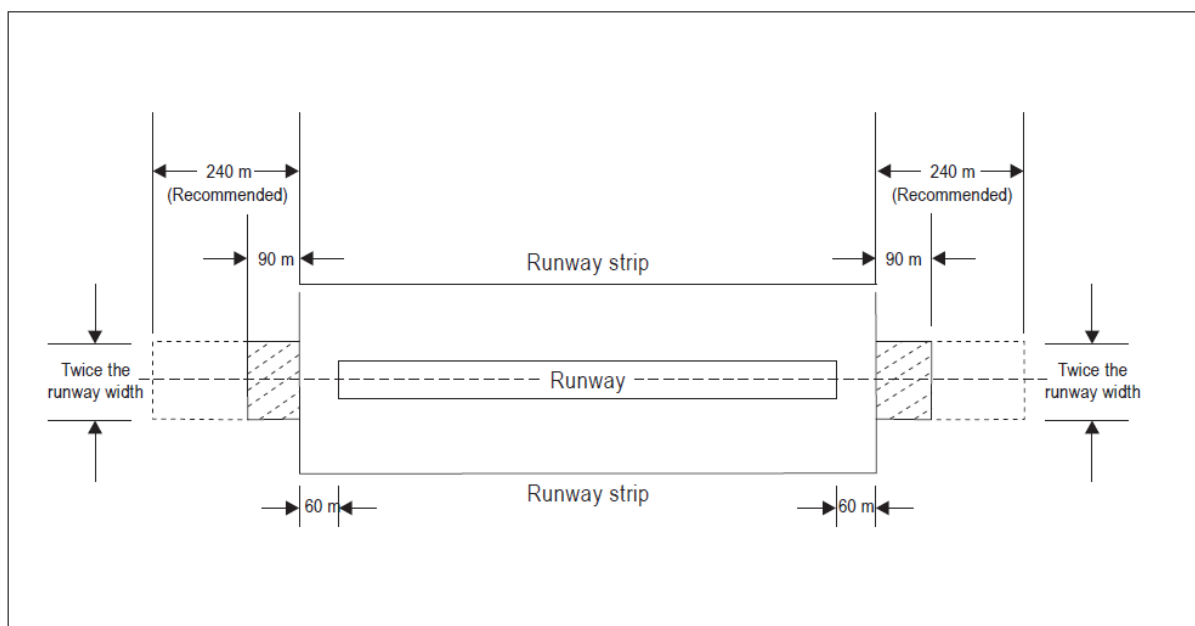
Figure A-5. Runway End Safety Area for a runway where the code is 3 or 4.
