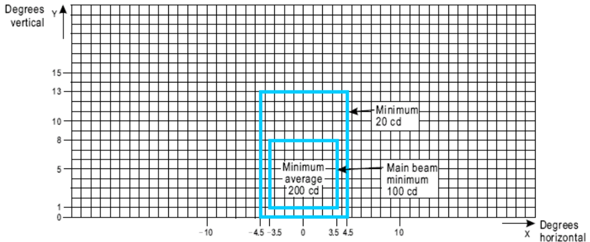
Figure A2-13. Isocandela diagram for taxiway centre line (15 m spacing), no entry bar and stop bar lights in straight sections intended for use in runway visual range conditions of less than a value of 350m
