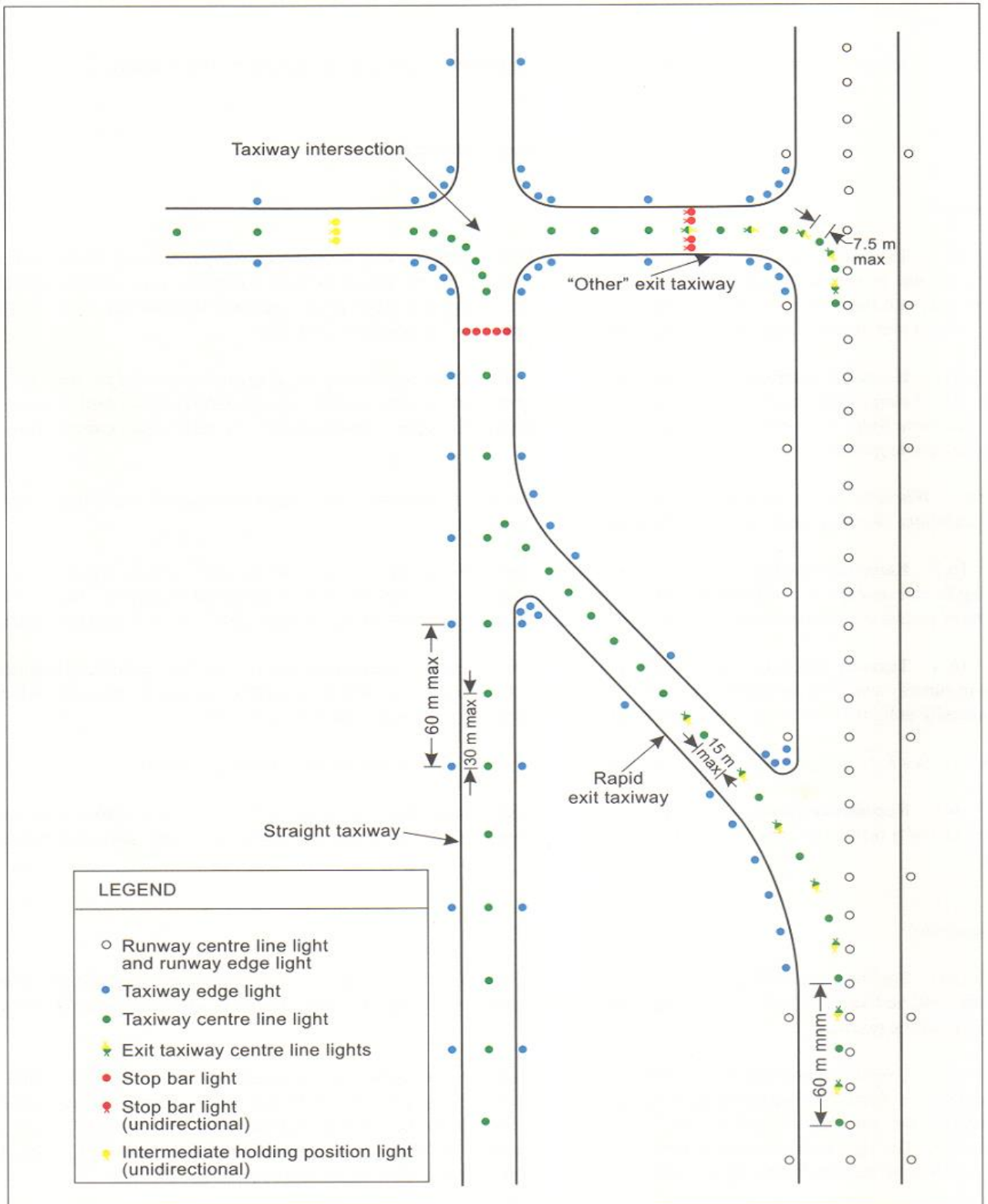
Figure 5-26. Taxiway lighting
