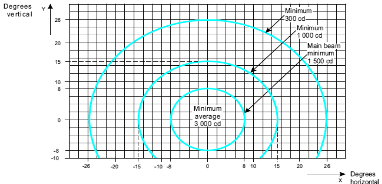
Figure A2-25. Isocandela diagram for each light in high-intensity runway guard lights, Configuration A
