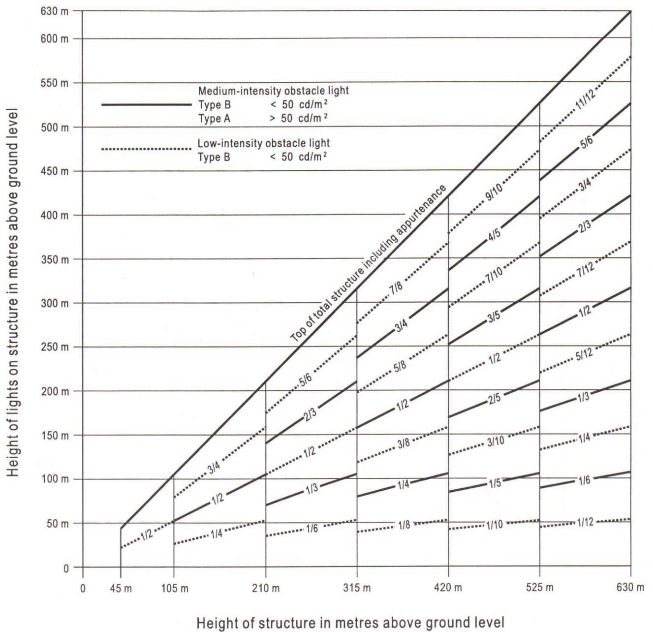
Figure A5-4. Medium-intensity dual obstacle lighting system, Type A/Type B
