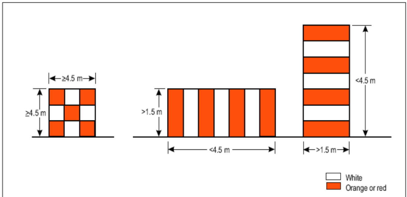
Figure 6-1. Basic marking patterns
