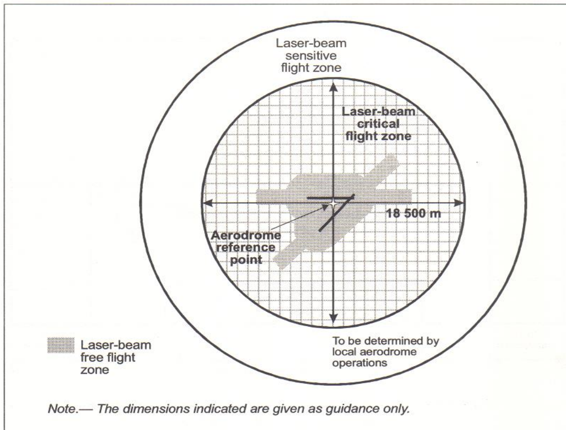
Figure 5-11. Protected flight zones
