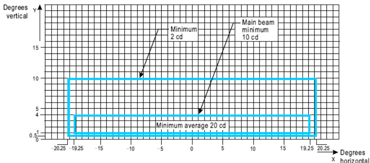
Figure A2-16. Isocandela diagram for taxiway centre line (7.5 m, 15 m, 30 m spacing), no-entry bar and stop bar lights in curved sections intended for use in runway visual range conditions of 350 m or greater
