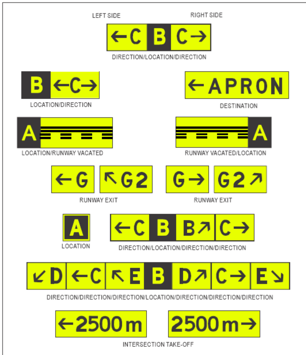
Figure 5-31. Information signs
