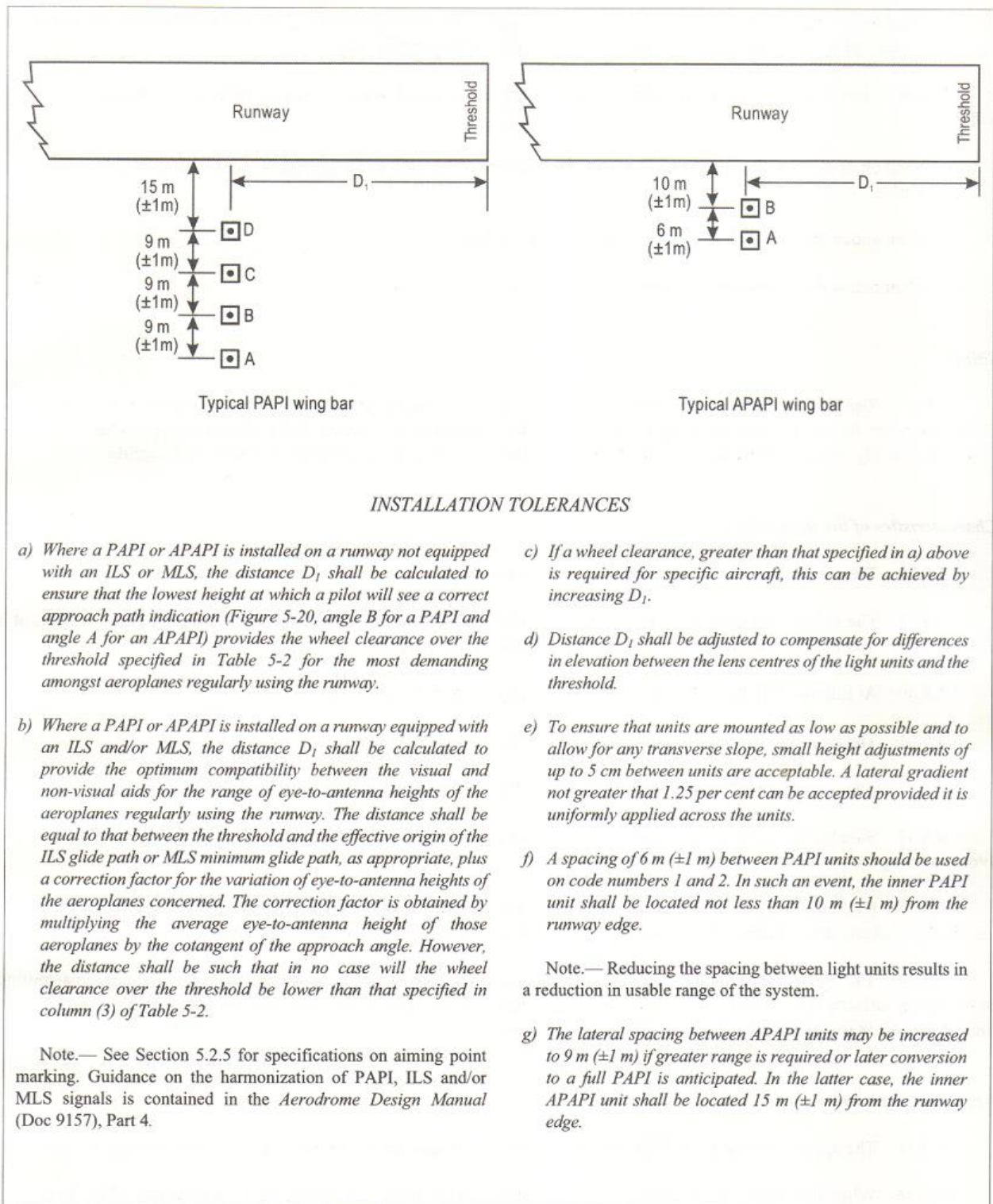
Figure 5-19. Siting of PAPI and APAPI
