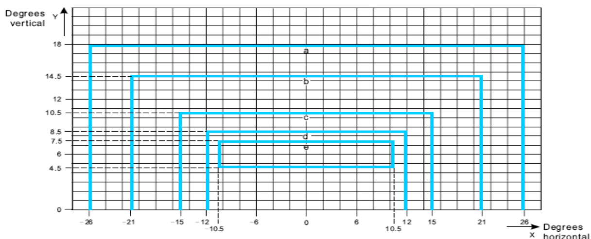
Figure A2-17. Isocandela diagram for high-intensity taxiway centre line (15 m spacing), no-entry bar and stop bar lights in straight sections intended for use in an advanced surface movement guidance and control system where higher light intensities are required and where large offsets can occur.
