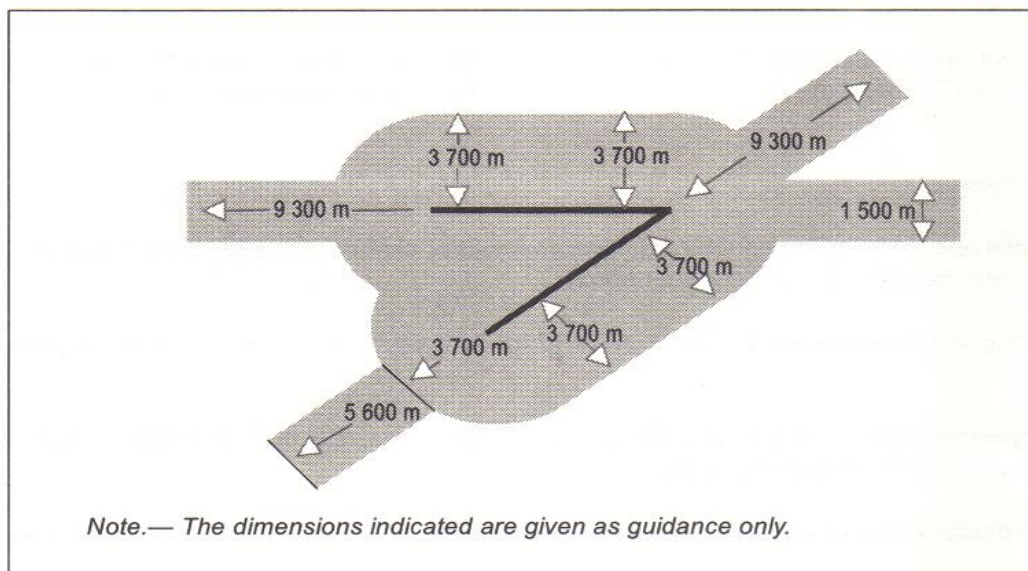
Figure 5-12. Multiple runway laser-beam free flight zone
