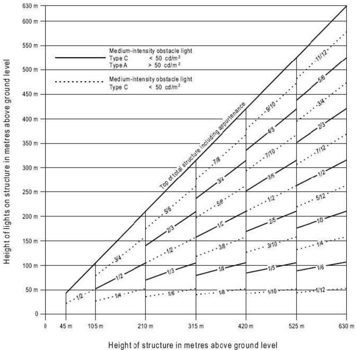
Figure A5-5. Medium-intensity dual obstacle lighting system, Type A/Type C
