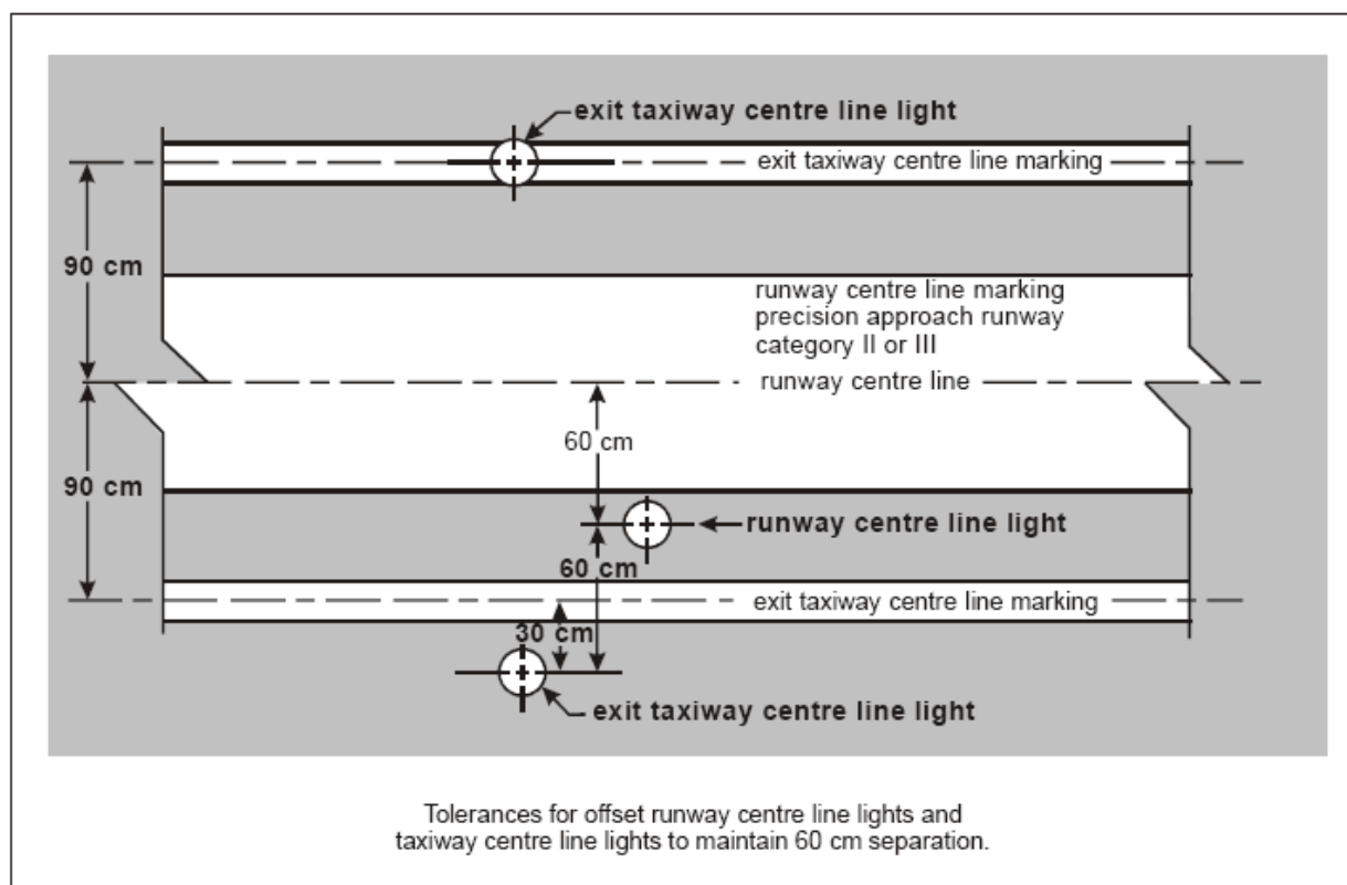
Figure 5-27. Offset runway and taxiway centre line lights
