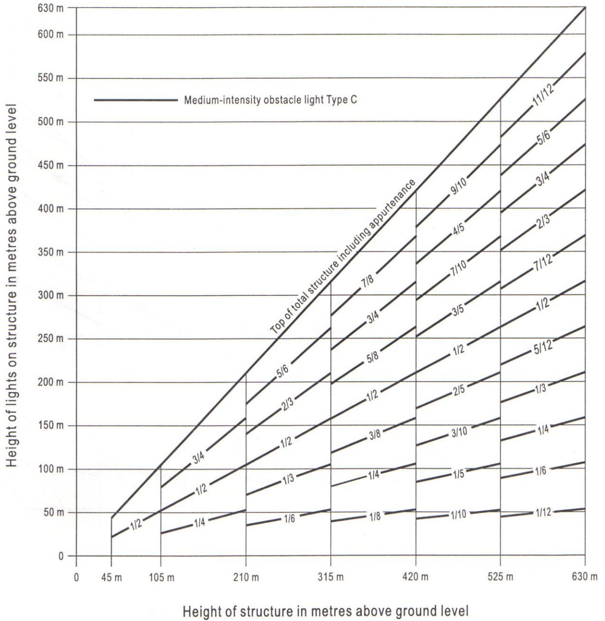
Figure A5-3 Medium Intensity Fixed red obstacle lighting system, Type C
