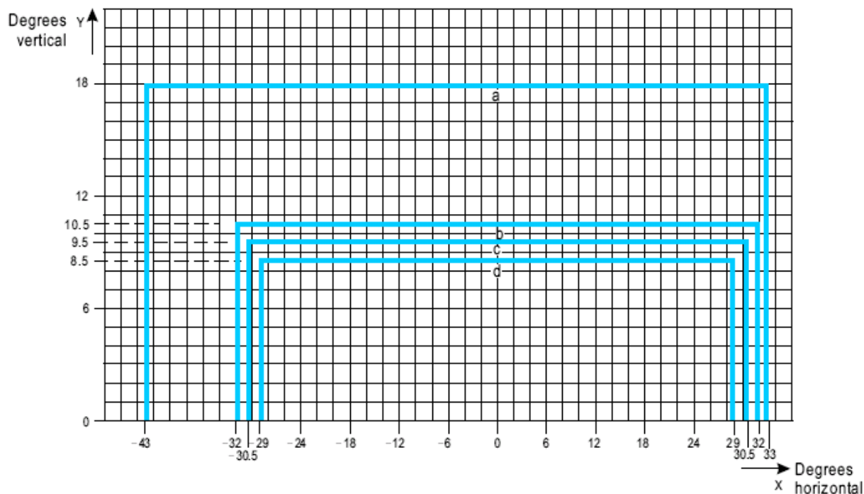
Figure A2-19. Isocandela diagram for high-intensity taxiway centre line (7.5 m spacing), no-entry bar and stop bar lights in curved sections intended for use in an advanced surface movement guidance and control system where higher light intensities are required
