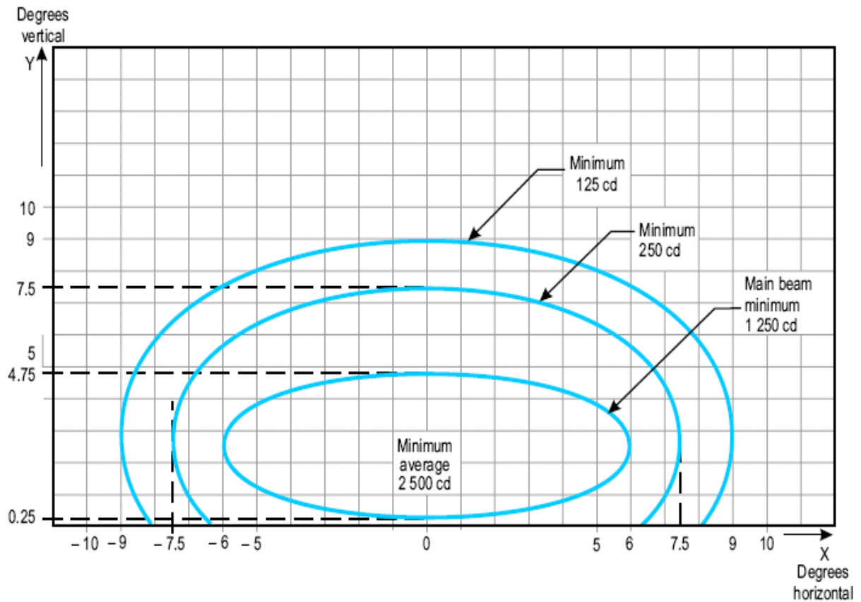
Figure A2-8. Isocandela diagram for runway end light (red light)
