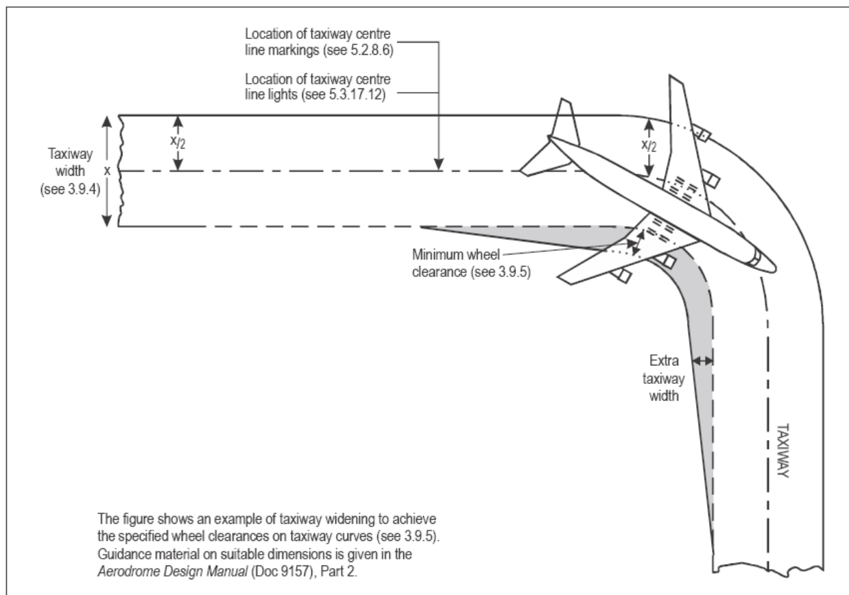
Figure 3-2. Taxiway curve
