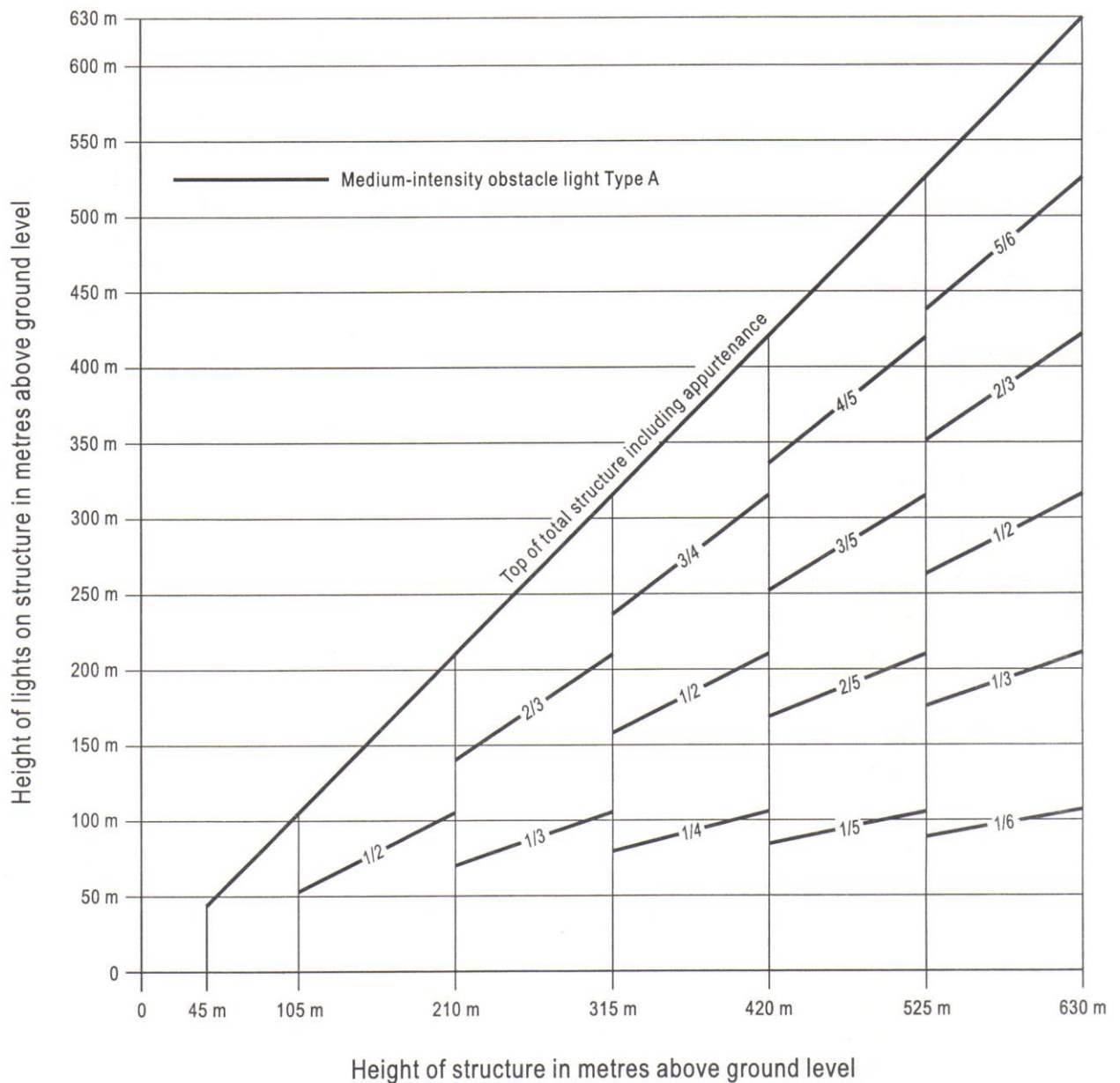
Figure A5-1. Medium-intensity flashing-white obstacle lighting system, Type A
