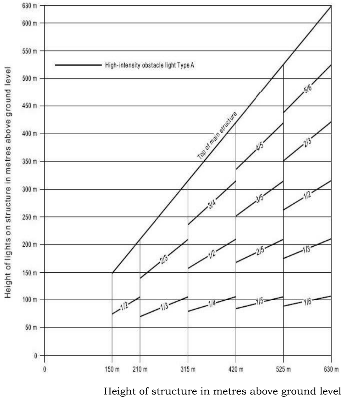
Figure A5-6. High-intensity flashing-white obstacle lighting system, Type A
