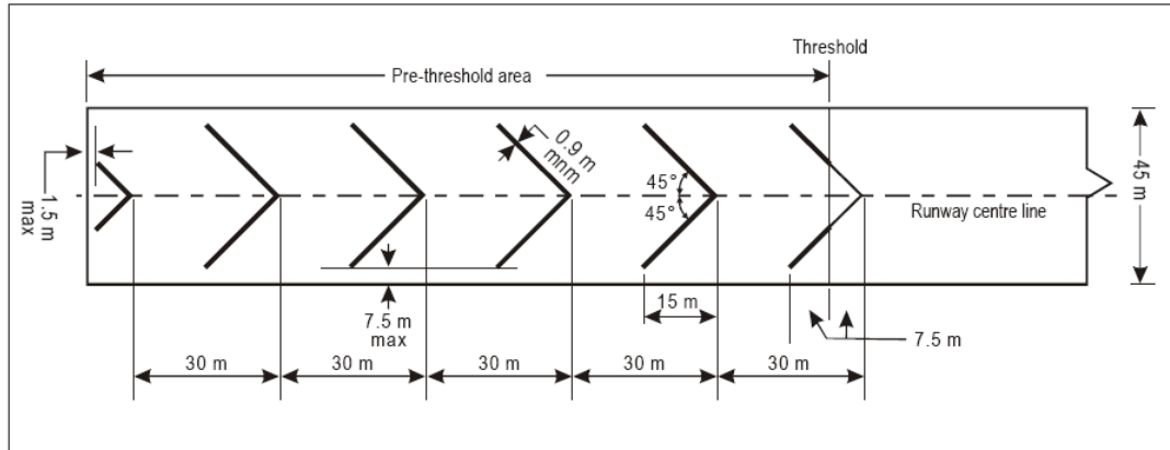
Figure 7-2. Pre-threshold marking
