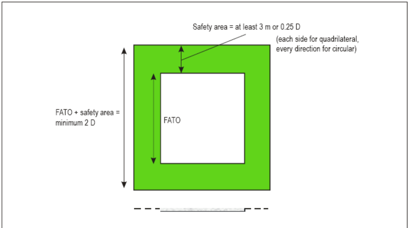
Figure 3-1. FATO and associated safety area
