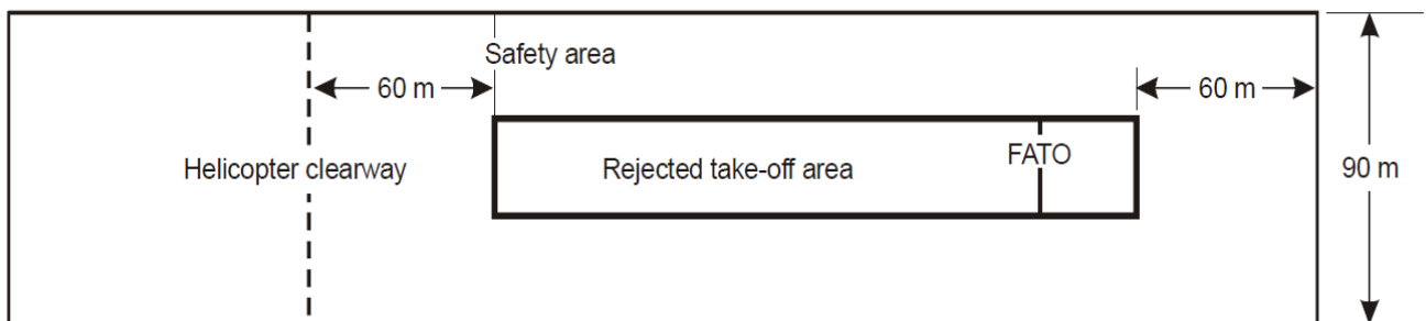
Figure A-1. Safety area for instrument FATO
