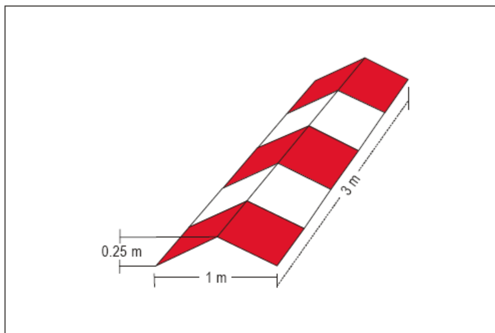
Figure 5-5. Runway-type FATO edge marker
