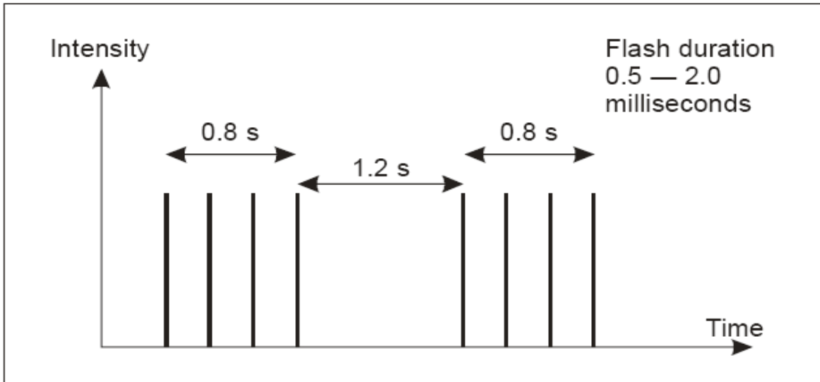
Figure 5-10. Heliport beacon flash characteristics
