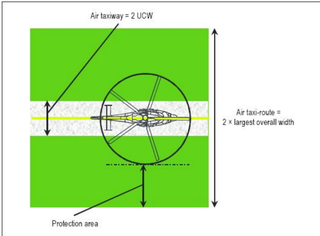
Figure 3-3. Helicopter air taxi-route/taxiway
