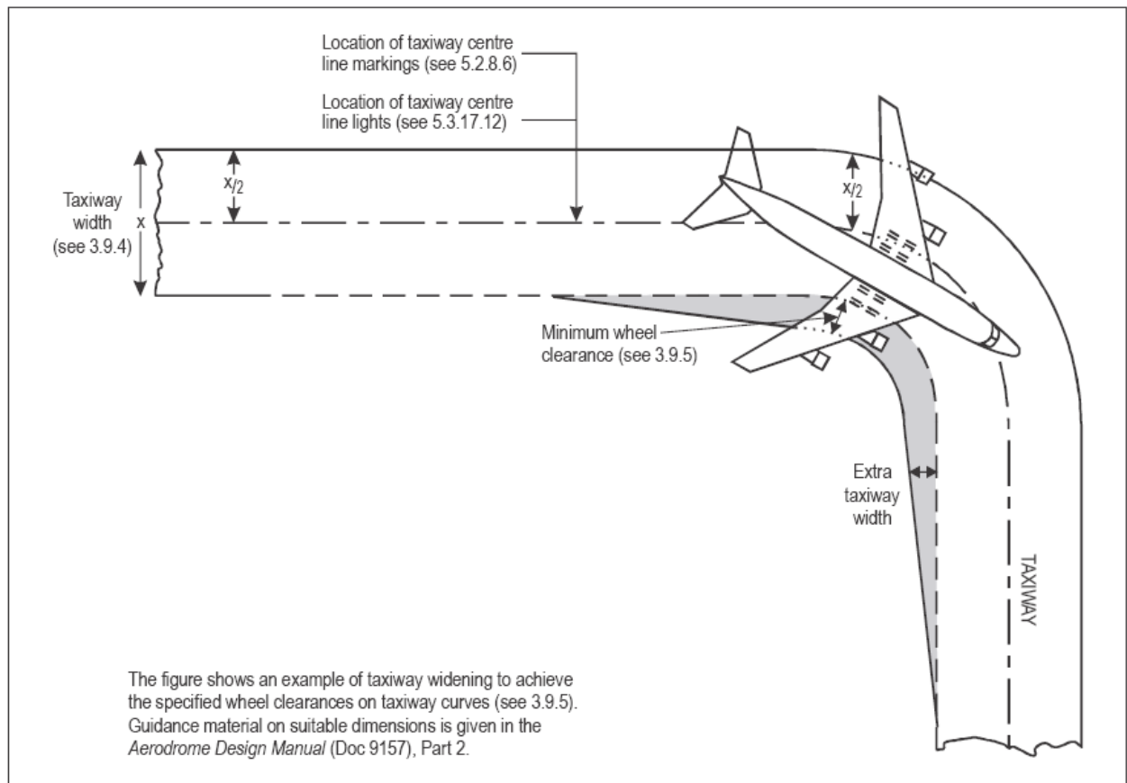
Figure 3-2. Taxiway curve
