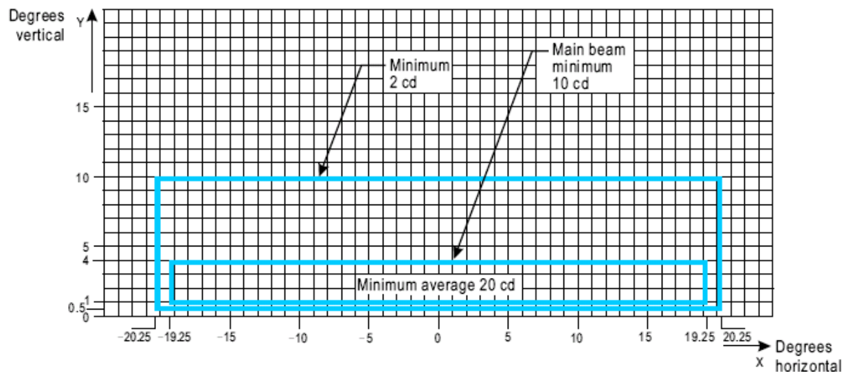
Figure A2-16. Isocandela diagram for taxiway centre line (7.5 m, 15 m, 30 m spacing), no-entry bar and stop bar lights in curved sections intended for use in runway visual range conditions of 350 m or greater
