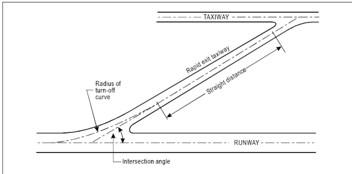
Figure 3-3. Rapid exit taxiway
