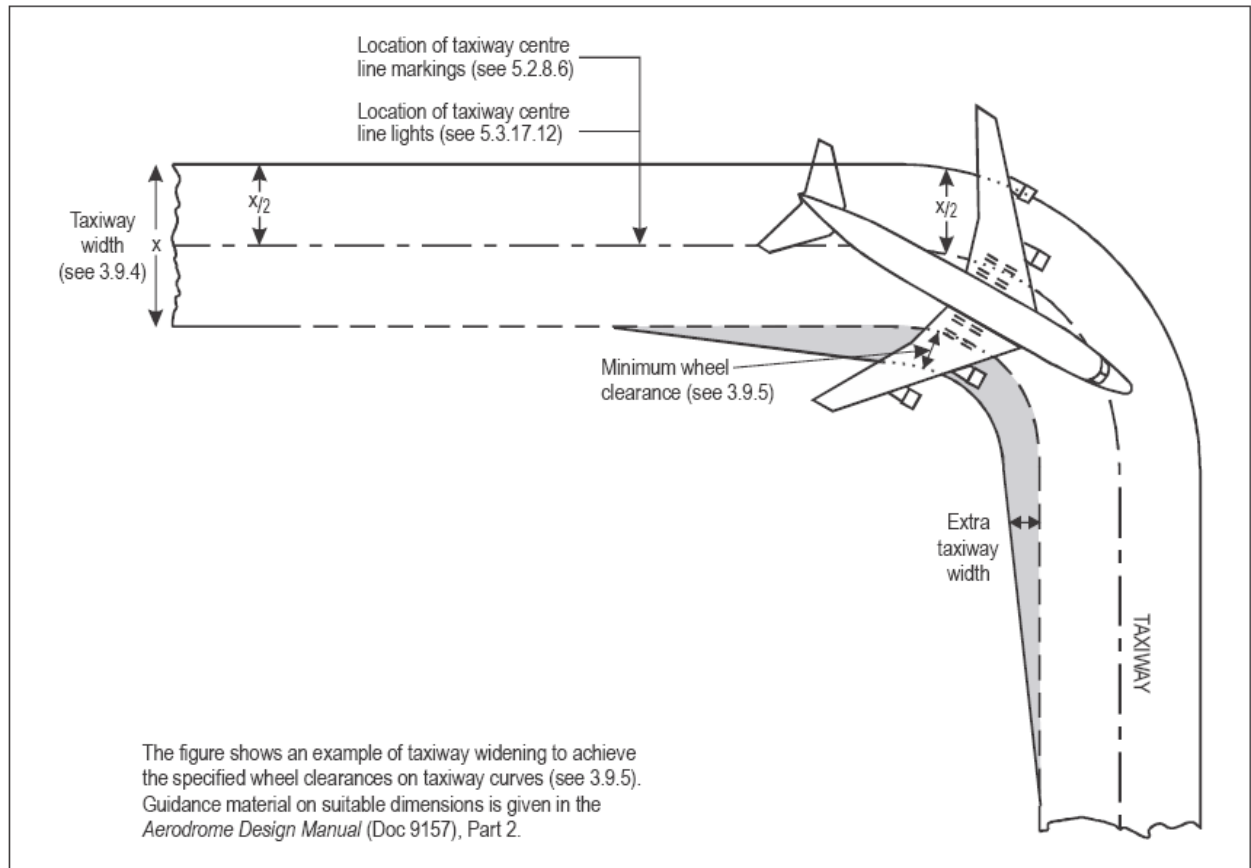
Figure 3-2. Taxiway curve
