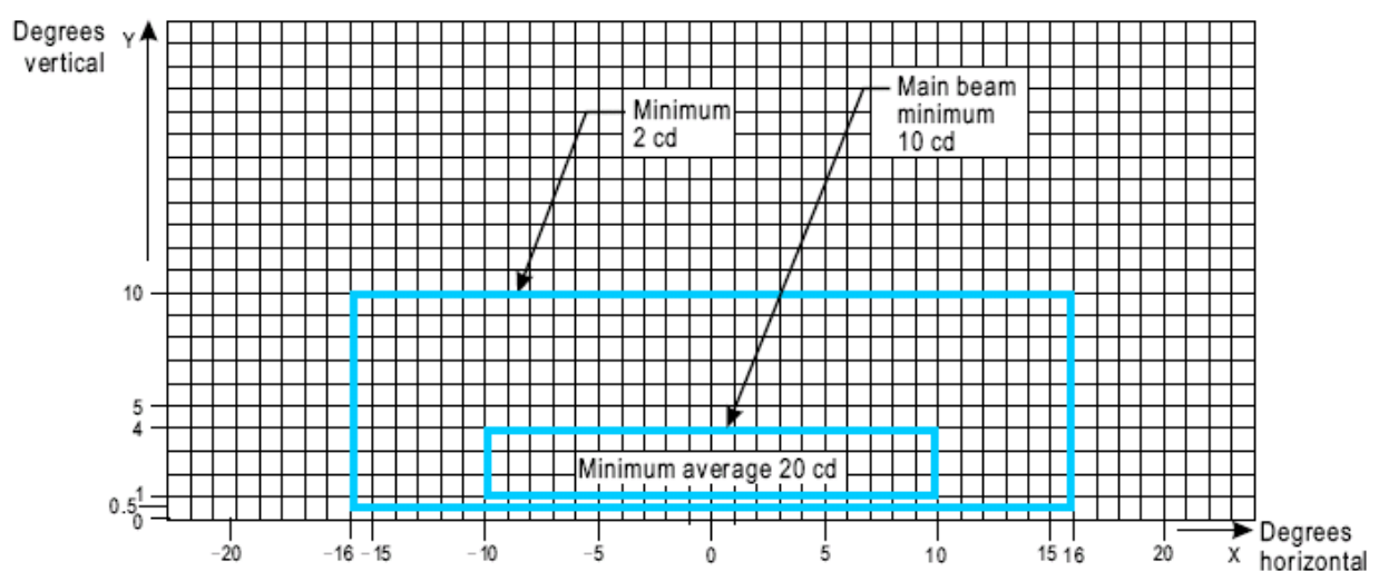
Figure A2-15. Isocandela diagram for taxiway centre line (30 m, 60 m spacing), no-entry bar and stop bar lights in straight sections intended for use in runway visual range conditions of 350 m or greater
