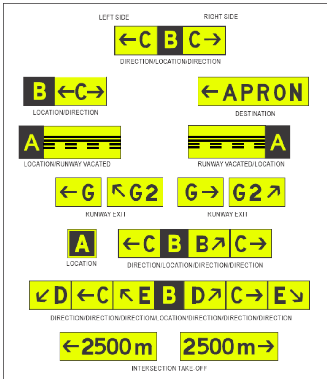
Figure 5-31. Information signs
