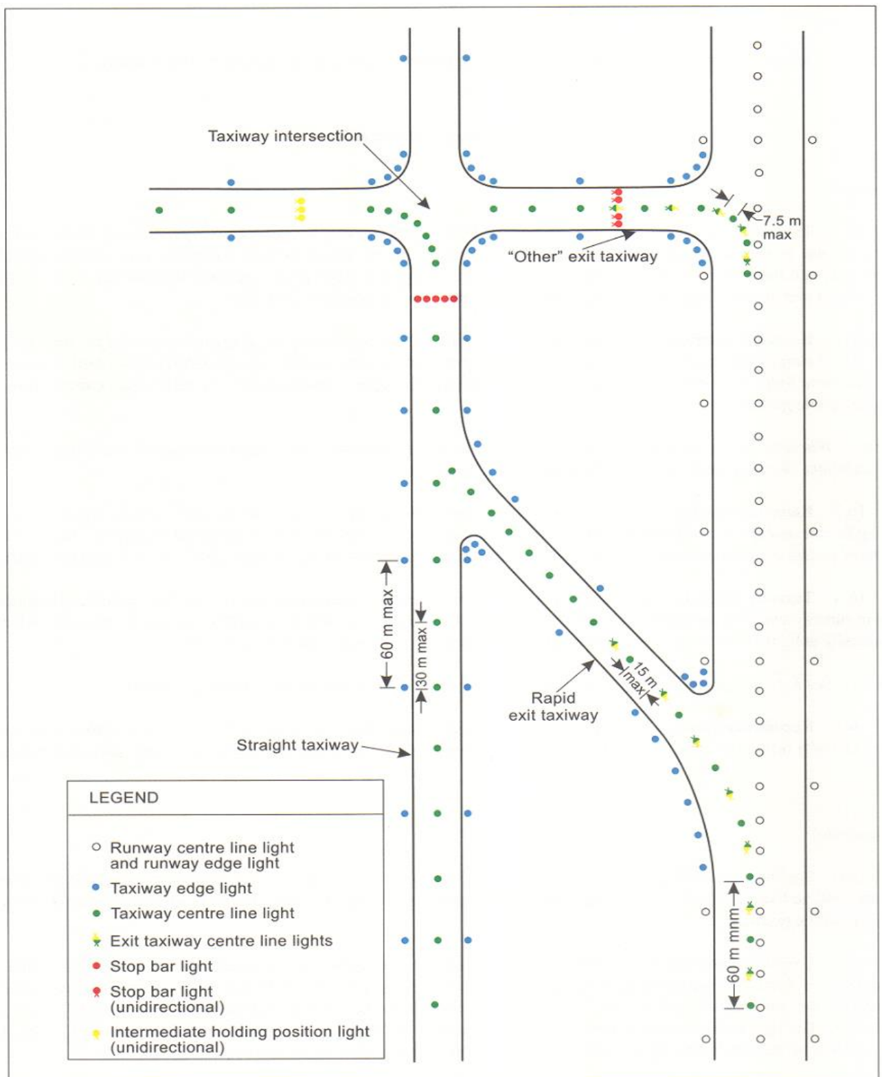
Figure 5-26. Taxiway lighting
