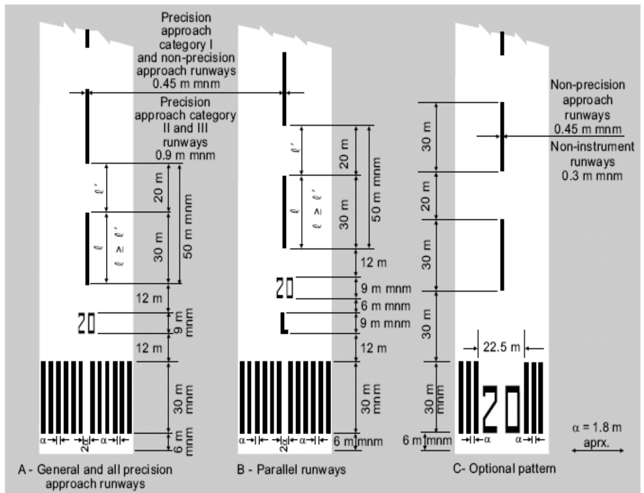
Figure 5-2. Runway designation, centre line and threshold markings
