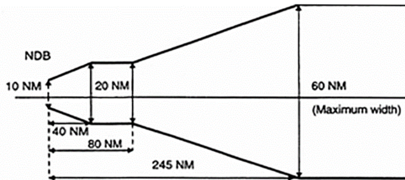
Corridor width from an NDB
