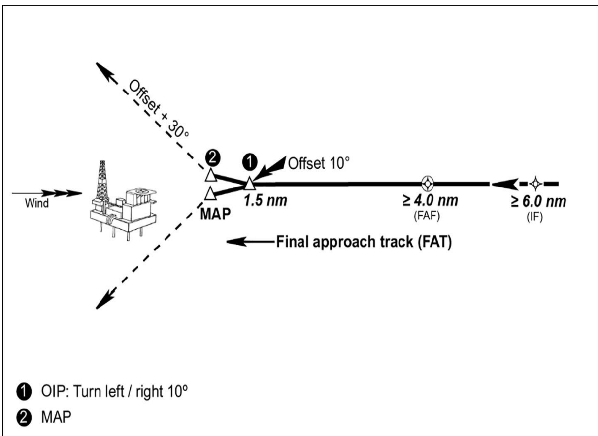
Figure 1 — Horizontal profile
