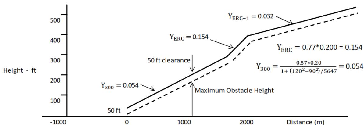
Figure 3 Assumed engine failure height less than 200 ft
