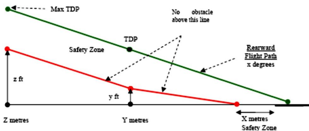
Figure 1 Rearward flight path
