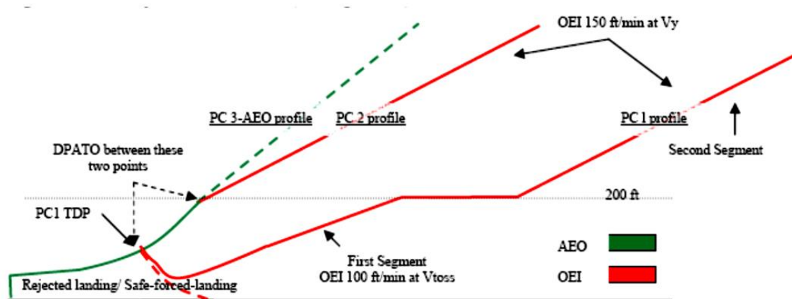
Figure 1 All Performance Classes (a comparison)
