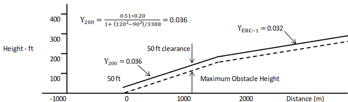
Figure 2 Assumed engine failure height 200 ft
