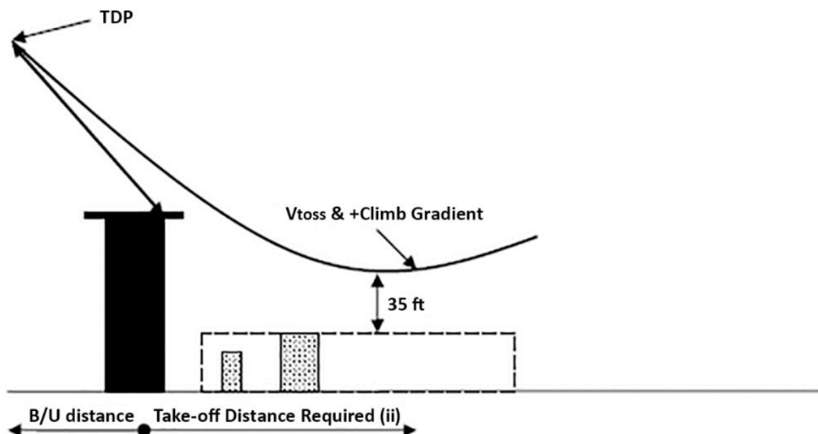
Figure 4 Elevate Helipad take-off
