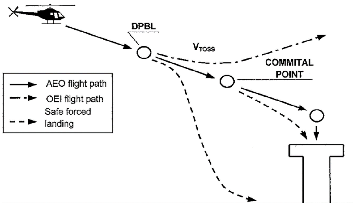
Figure 4 Typical landing profile PC2 to a helideck/elevated FATO, non-hostile environment
