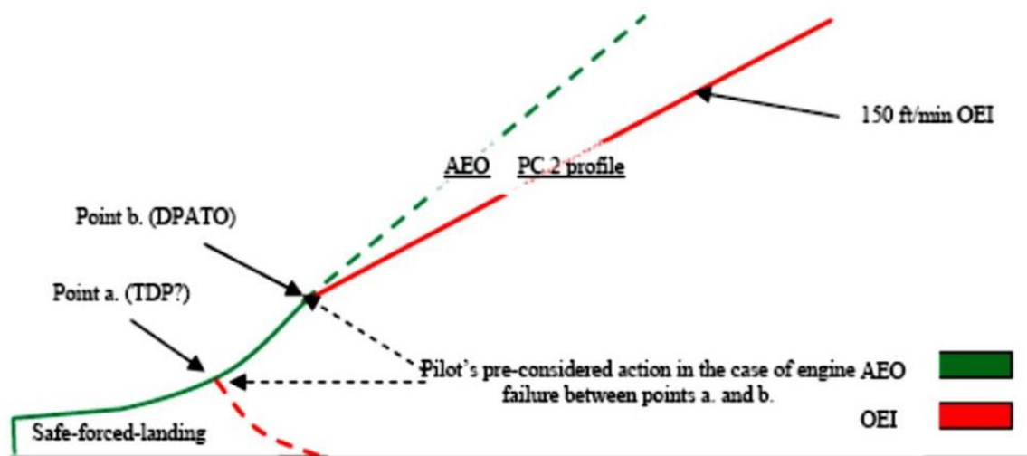
Figure 5 The three elements in a PC 2 take-off
