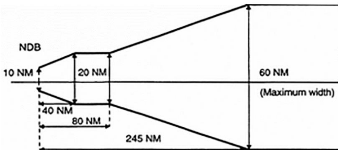
Figure 2 Corridor width from an NDB
