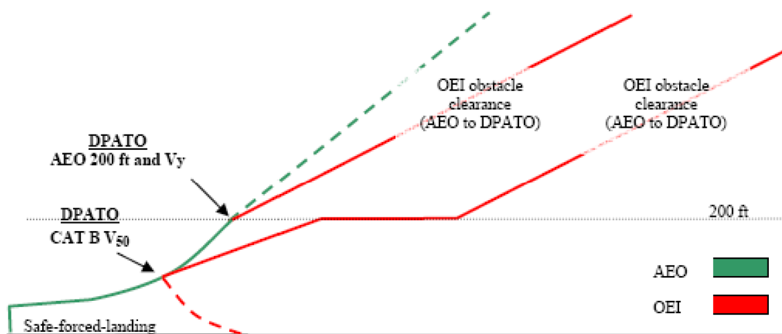
Figure 7 Suggested AEO locations for DPATO
