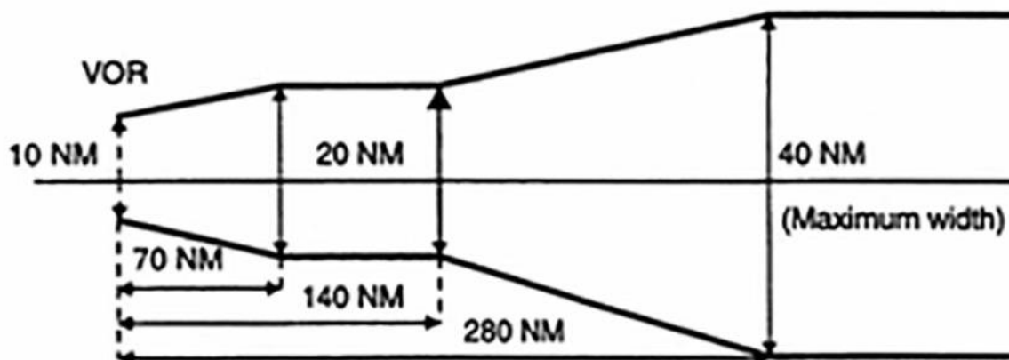
Figure 1 Corridor width from a VOR station
