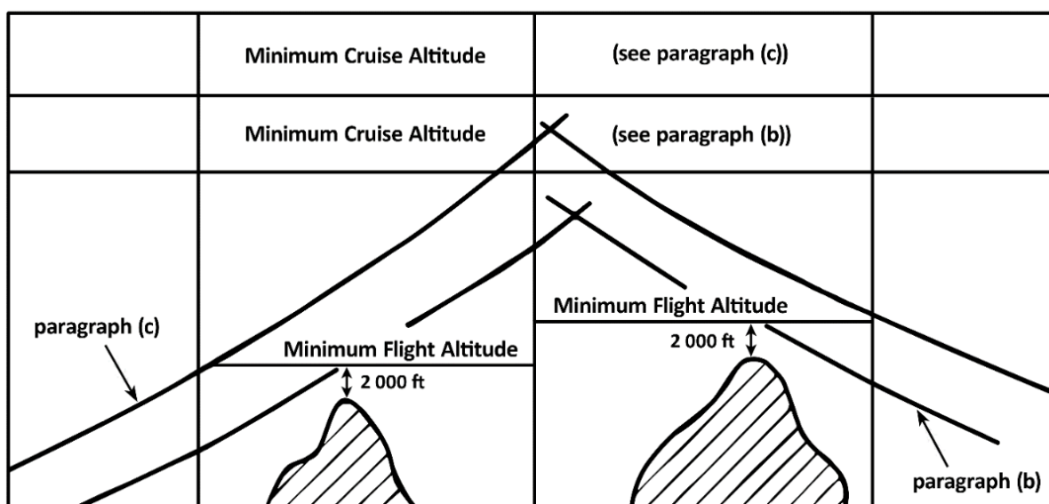
Figure 1 Intersection of the two drift down paths
