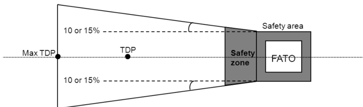
Figure 2 Obstacle accountability
