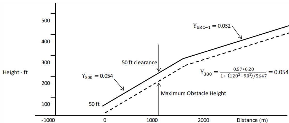
Figure 1 Assumed engine failure height 300 ft
