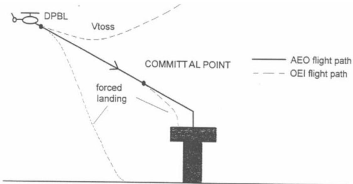
Figure 2 Standard landing profile
