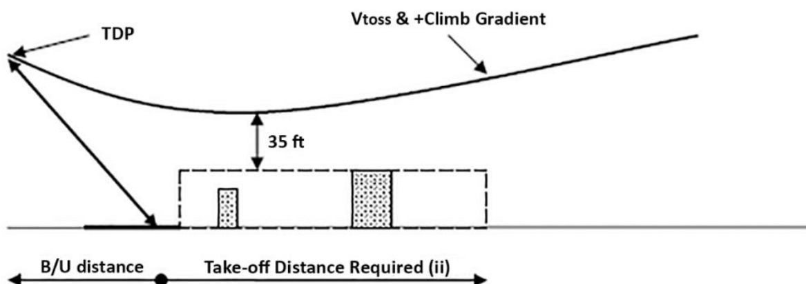
Figure 3 Helipad take-off
