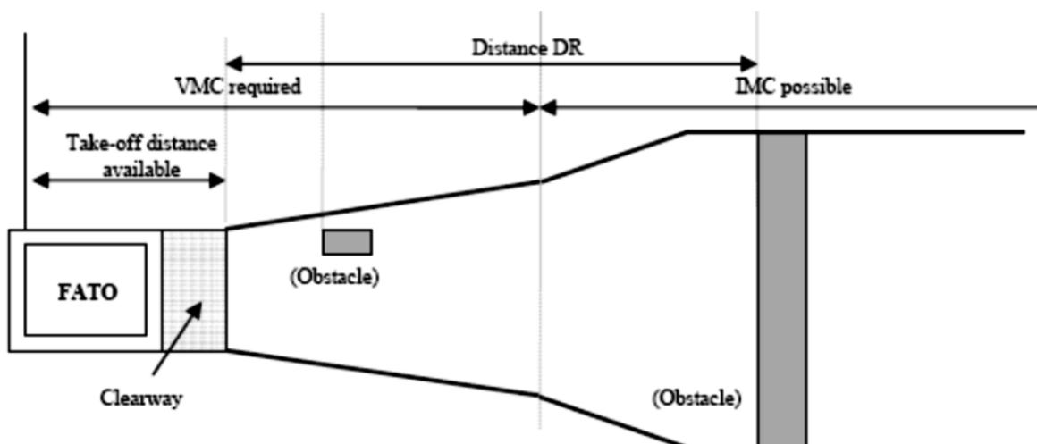
Figure 4 Performance Class 2 Obstacle Clearance (plan view)
