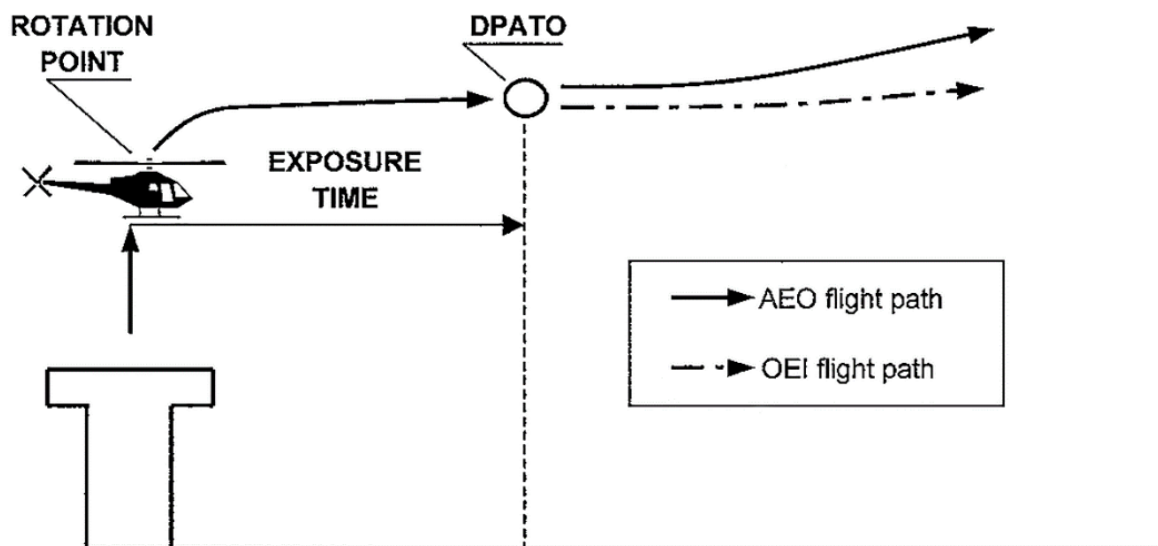
Figure 3 Typical take-off profile PC2 from a helideck/elevated FATO, non-congested hostile environment
