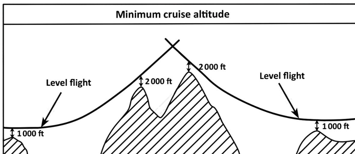
Figure 1 Intersection of the drift down paths
