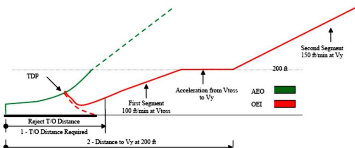
Figure 2 Performance Class 1 distances
