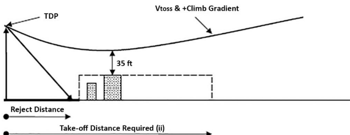
Figure 2 Short Field take-off
