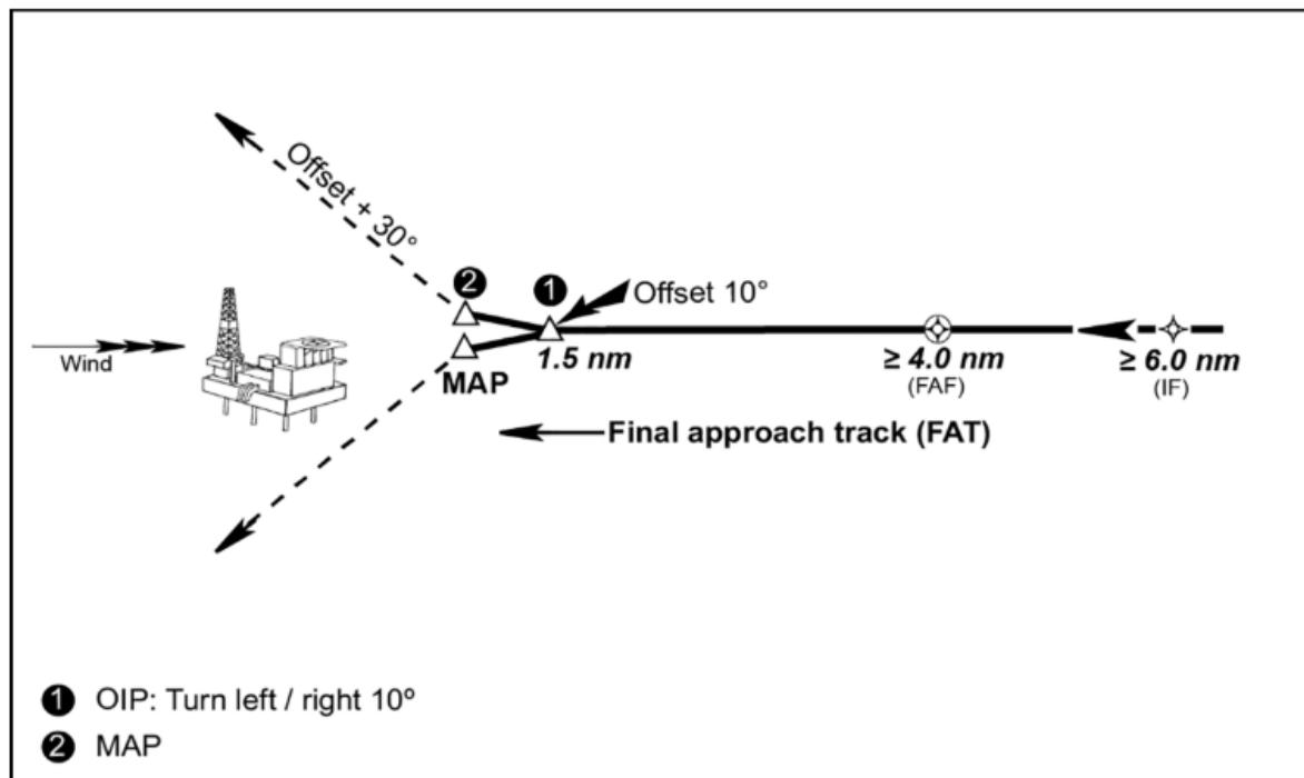
Figure 1 — Horizontal profile
